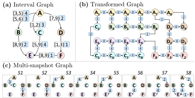
Figure 1: Transit network as a temporal graph.
